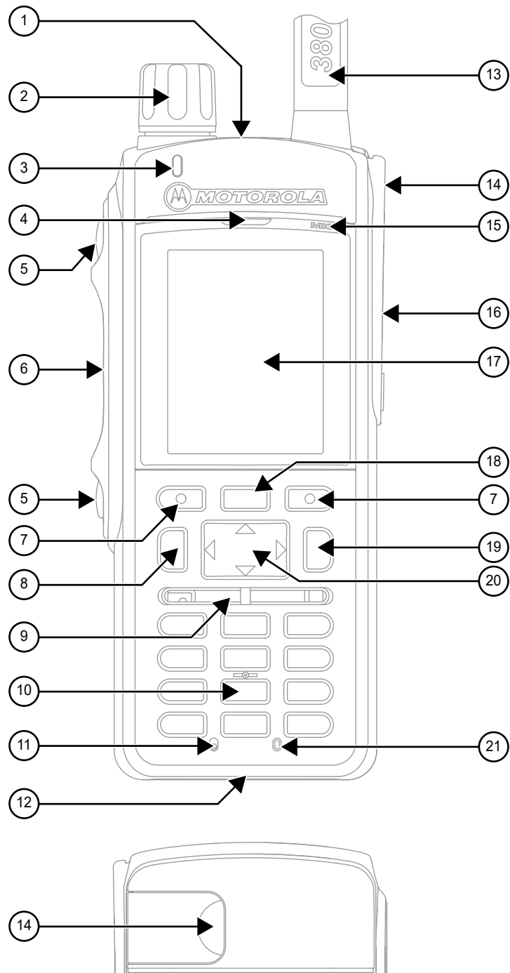
Figure 15: MTP6650 Controls and Indicators
